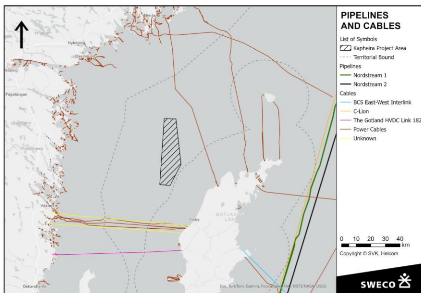
Figure 39. Pipelines and cables within and around the Kapheira area.
