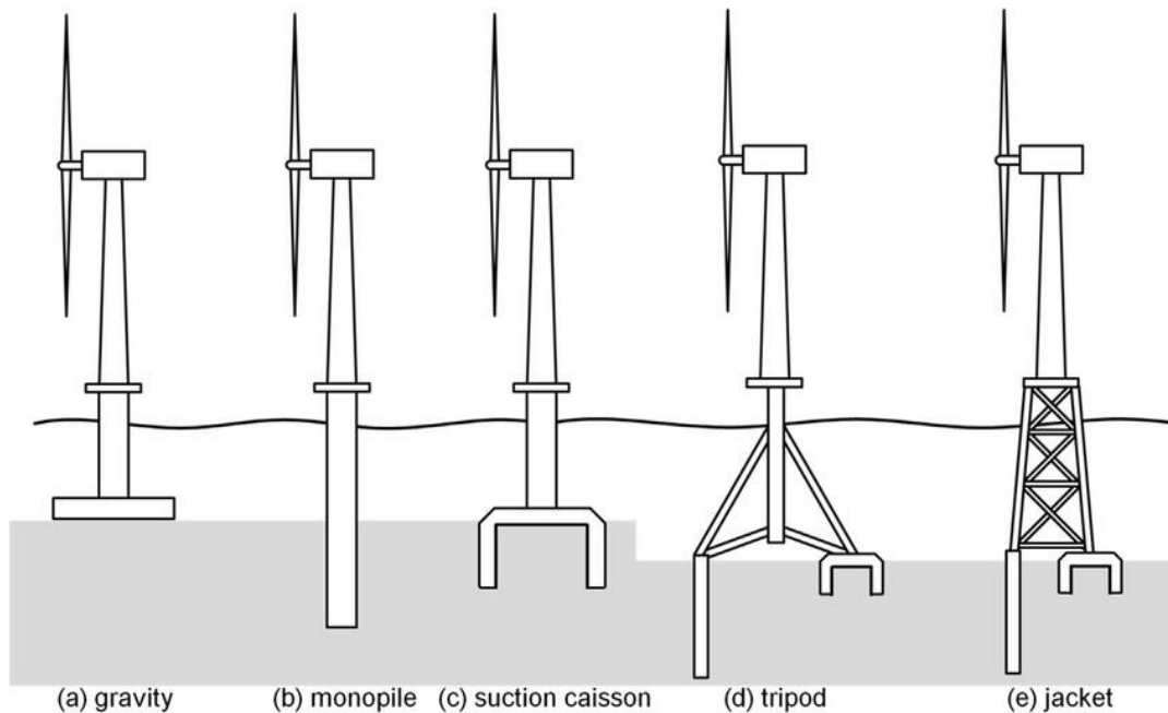
Figure 7. Examples of different foundation types, its attachment, and combinations of attachments (Oh et al. 2018).
