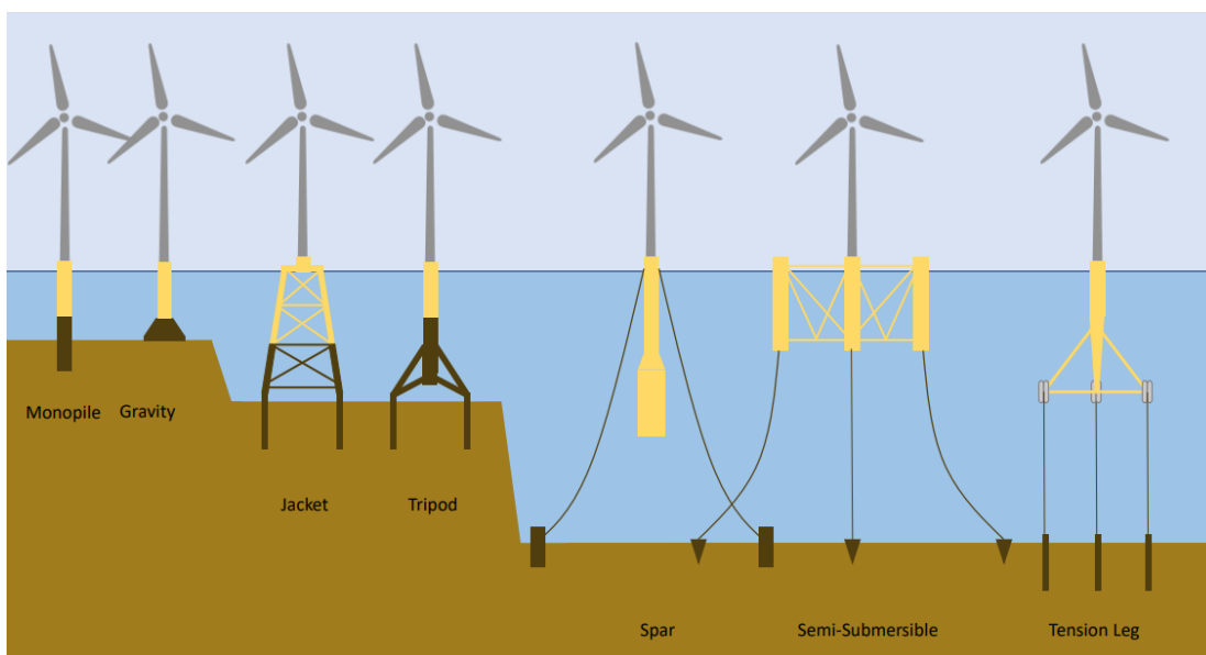
Figure 5. Common types of foundation for offshore wind power sites (Dornhelm 2019).
