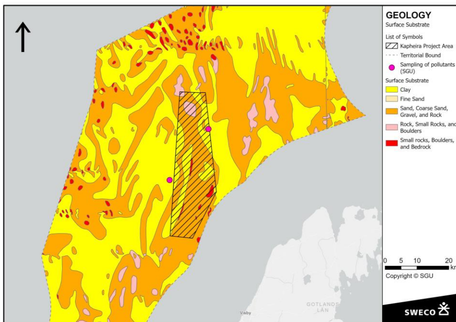
Figure 26. The map shows the project area of Kapheira with expected bottom substrate classified by SGU. It also marks two of SGU's sampling stations for metals and organic pollutants. Data has been collected from Hallberg et al. (2010) and Swedish Environmental Monitoring, data host SGU (2023a and 2023b)
