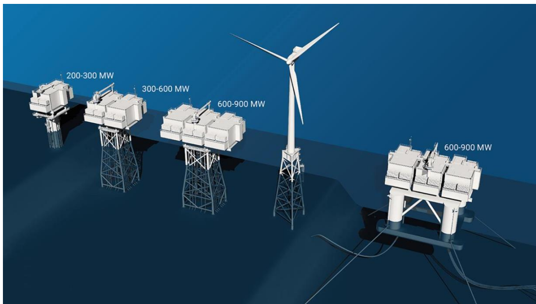
Figure 4. Schematic examples of substations and foundation types (Dodd, 2017).
