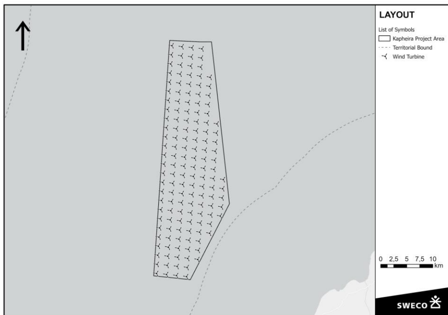
Figure 2. Kapheira with a layout example of 143 wind turbines.
