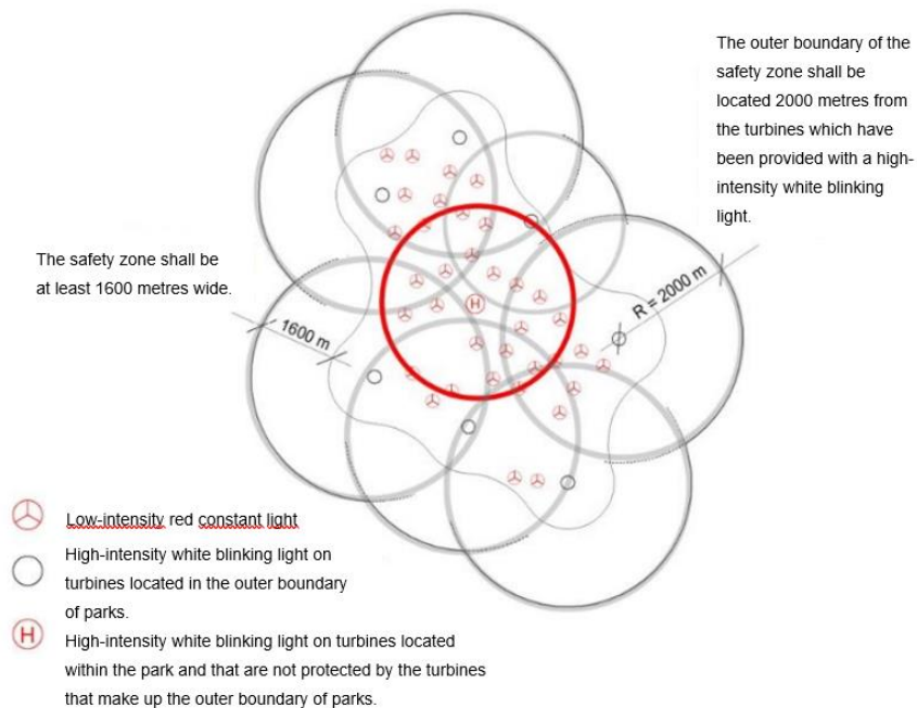
Figure 12. Method for marking wind turbines that, including the rotor in its highest position, have a height of over 150 meters above ground or the water surface (Swedish Transport Agency).
