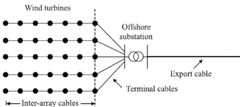
Figure 9. Schematic overview of the internal cable network, offshore substation, and the export cable. (Rentschler et al. 2020).
