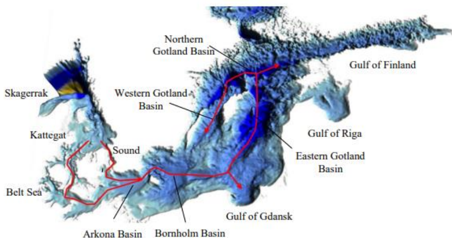
Figure 29. Bathymetric map of the southern Baltic Sea and the path of water flow during inflows from Öresund and the Belt Sea through the Baltic Sea (red arrows). The figure is sourced from Hansson and Viktorsson 2023.
