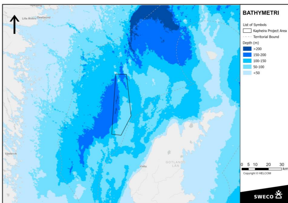
Figure 25. Bathymetry over the area surrounding Kapheira.
