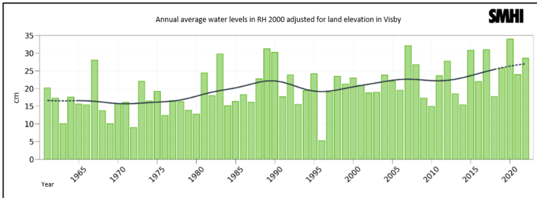
Figure 28. Water levels in Visby, SMHI (2023c). The bars show the annual average values of water levels in RH 2000 adjusted for land elevation in Visby. The grey line represents a moving average calculated over approximately ten years. The dashed section of the line indicates that the average is calculated over fewer years.
