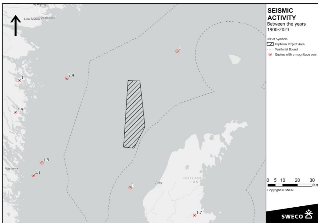
Figure 27. All earthquakes with a magnitude of at least 1, in and around the project area, which have been recorded from year 1900 until today (SNSN).
