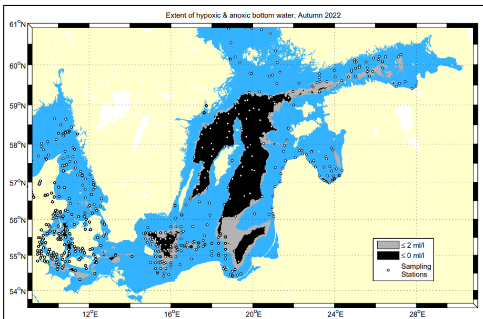
Figure 30. Oxygen deficiency in the bottom waters layers of the Baltic Sea during the autumn of 2022 (Hansson and Viktorsson 2023)
