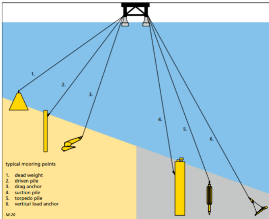
Figure 6. Illustration of the most common methods to moor floating foundations (X Castillo 2020).
