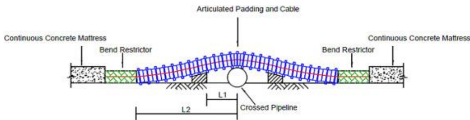
Figure 11. An example of the design of a secure crossing between pipes and cables (Reda et al. 2017).
