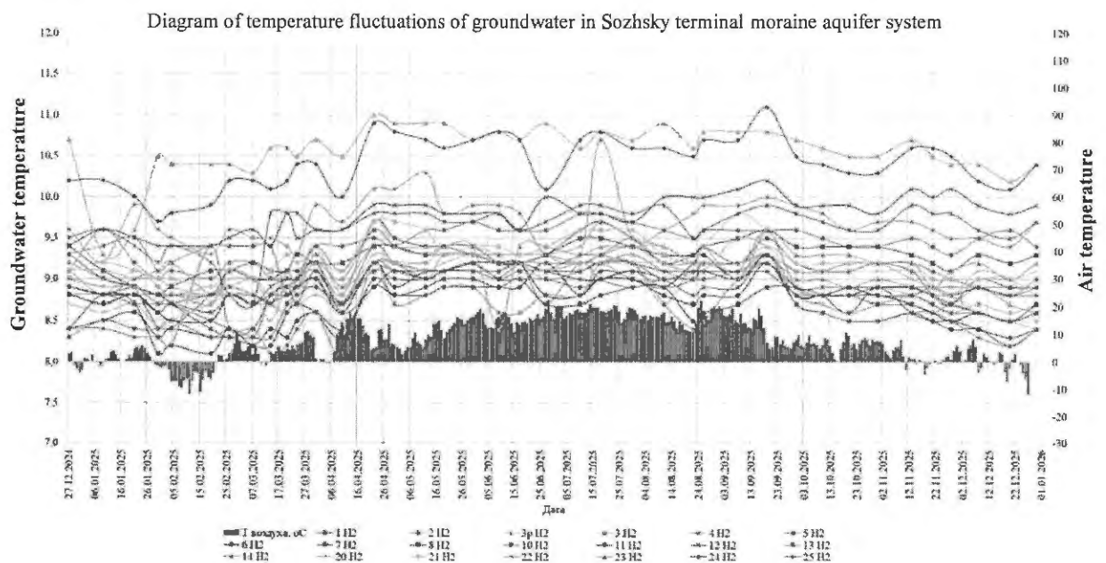
Figure 8.10 Chronological diagram of temperature fluctuations of groundwater in Sozhsky terminal moraine aquifer system in 2025
