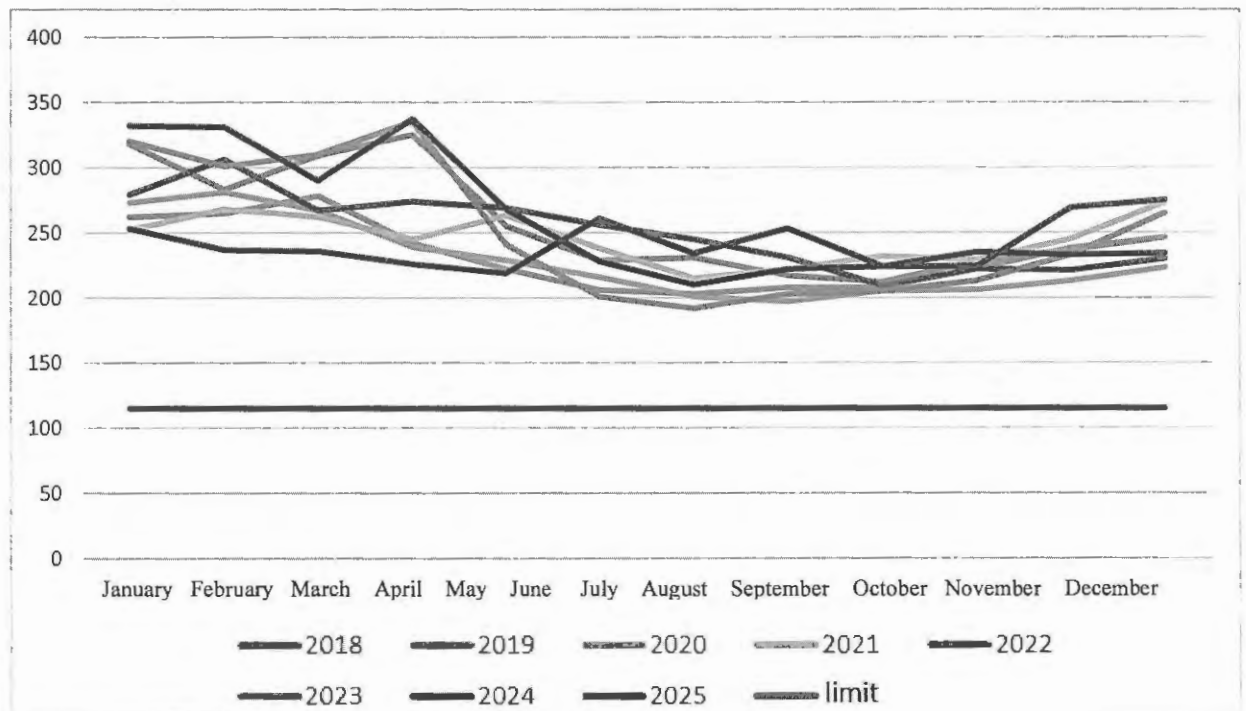
Figure 8.28 Graph of water level measurement at the water gauge station of the Viliya river (Malye Sviryanki settlement) in 2018-2025, m, BS
