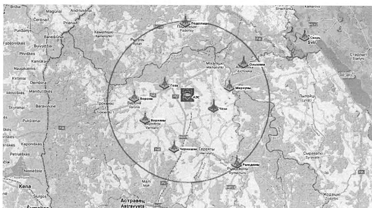
Figure 8.40 Belarusian NPP ACSRS RCP layout
