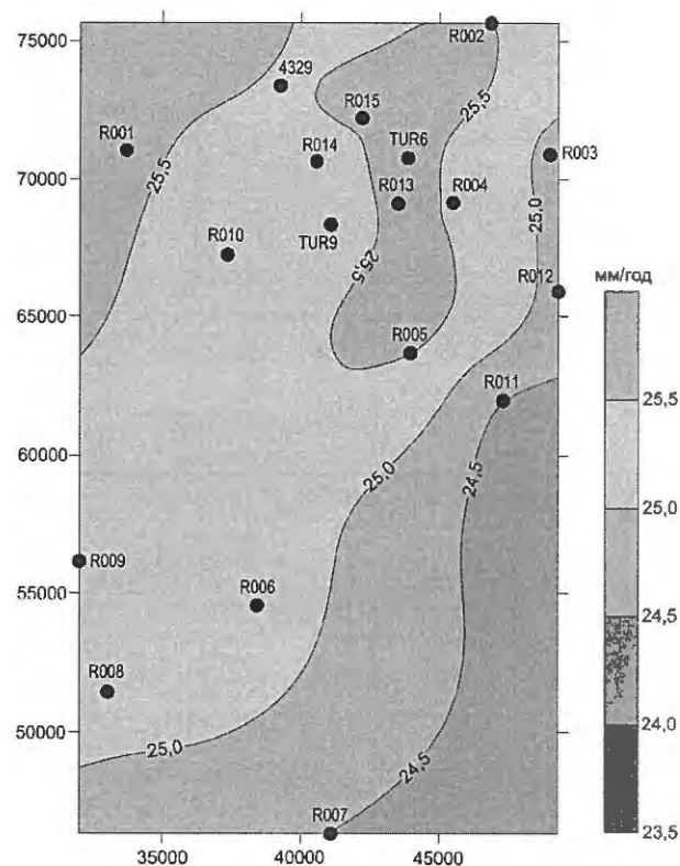
Figure 8.36 Distribution of velocities of horizontal motion of points recorded in 2012-2025
