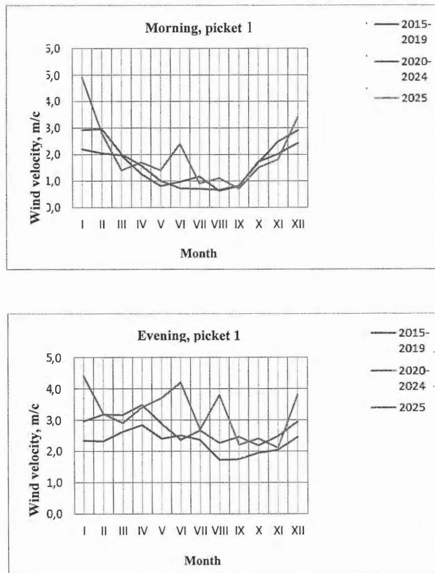
Figure 8.22 Combined wind velocity variation graphs at picket 1 over 2015-2019, 2020-2024 and 2025 observation periods
