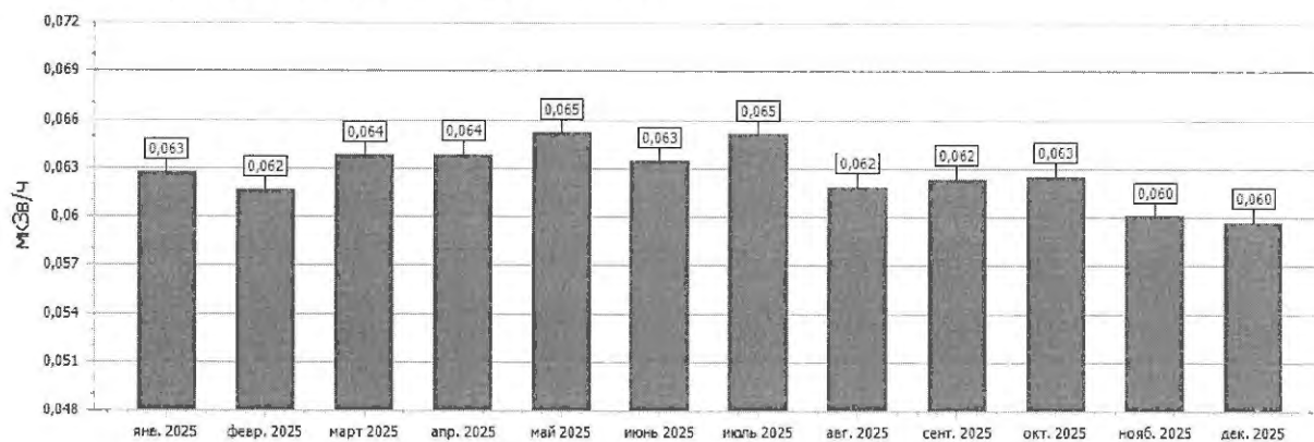
Figure 8.41 Average monthly values of ADER in 2025
