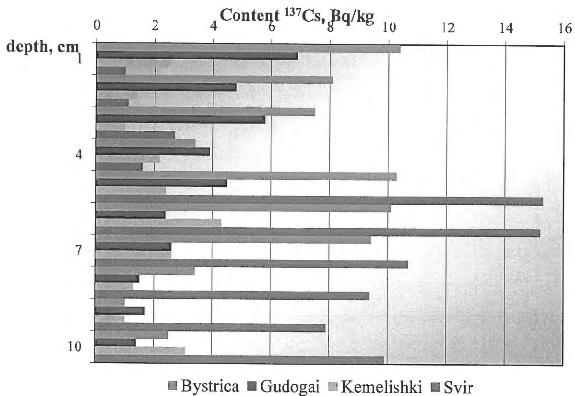
Figure 9.4 – Actual distribution of ^{137}\text{Cs} along the vertical profile of soils at LGTSs located in the area of the Belarusian NPP
