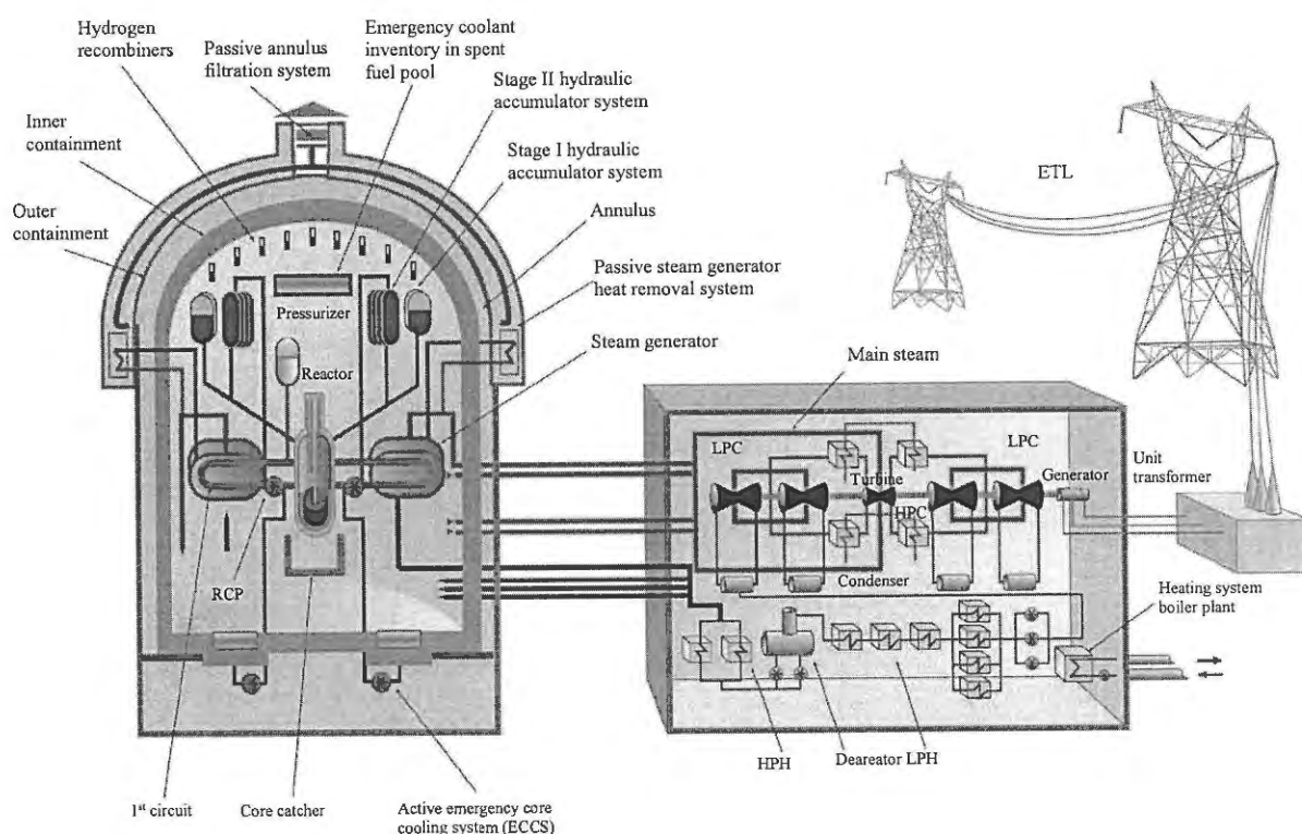
Figure 1.2 – NPP VVER-1200 power unit schematic diagram
