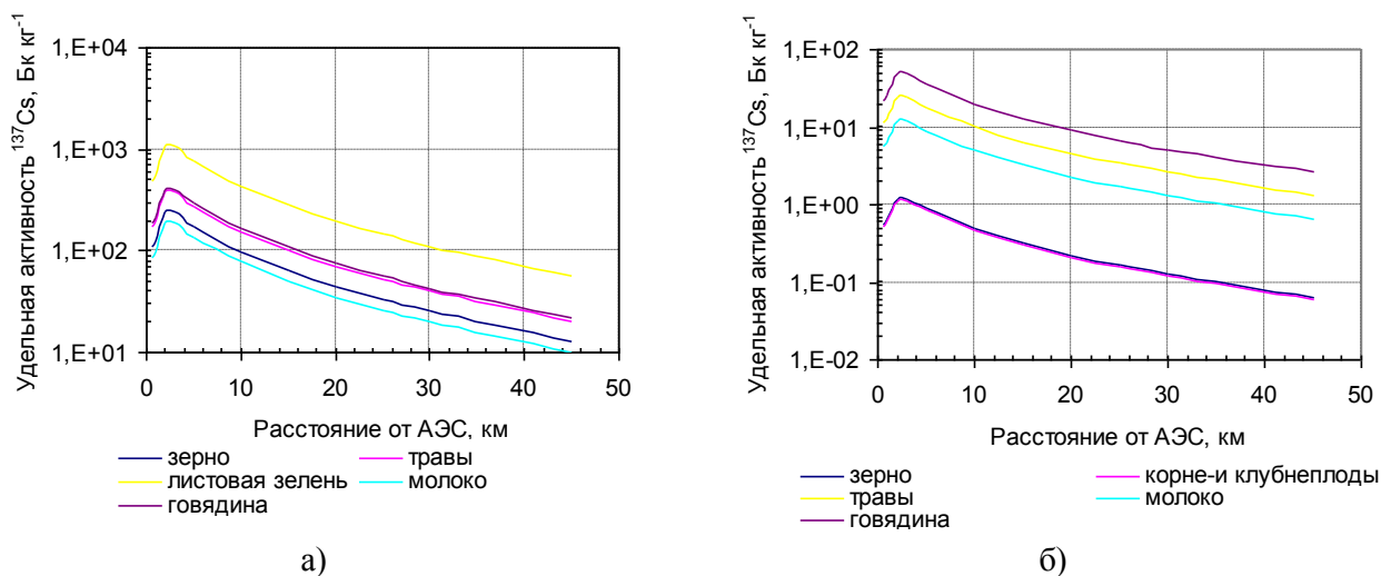
Figure 107 – Specific activity of ^{137}\text{Cs} in sorts of agricultural products within first (a) and the following vegetation season (б) after emergency fallouts
