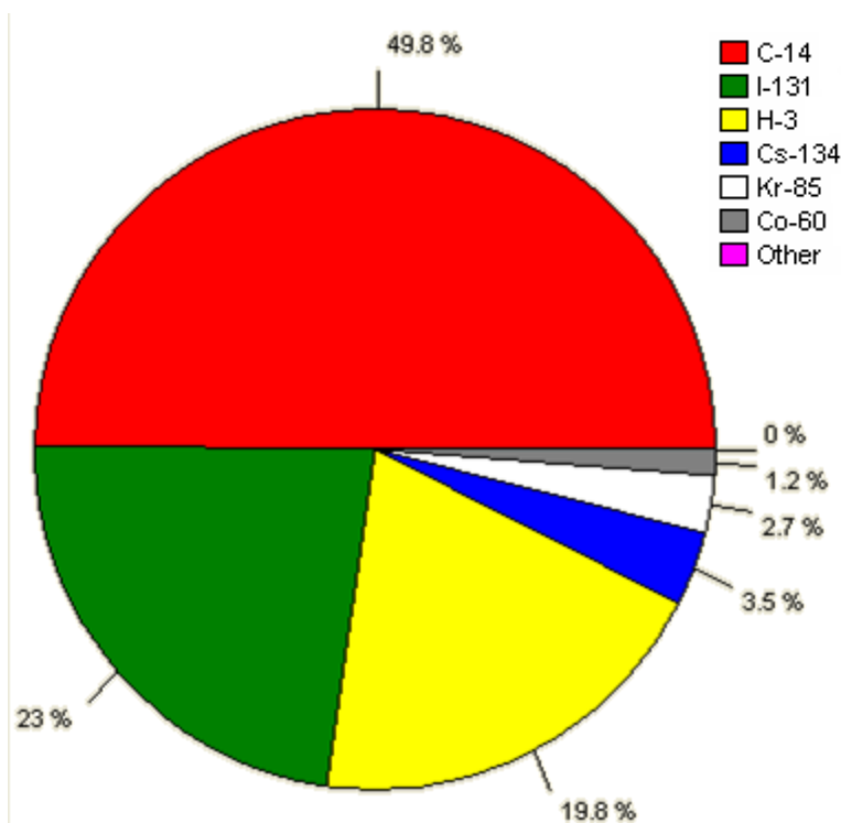
Figure 141 – Contribution of various radio nuclides into the total dose
