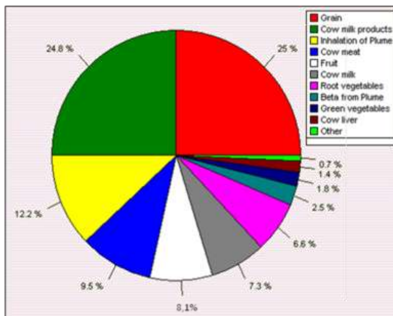
Figure 144 – Contribution of various ways of irradiation into total dose
