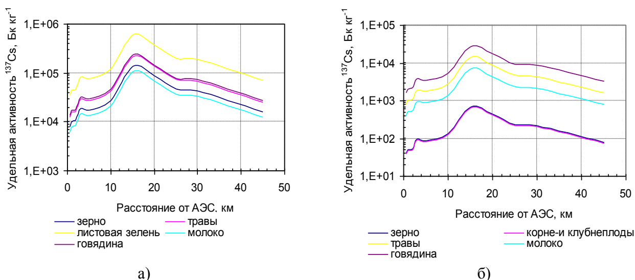
Figure 104 – Specific activity of ^{137}\text{Cs} in sorts of agricultural products within first (a) and following vegetation seasons (b) after emergency fallouts
