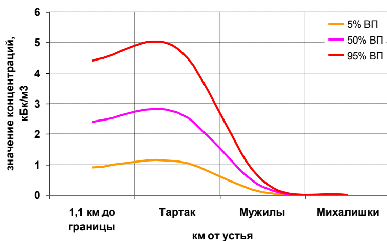
Figure 100 - Dynamics changing concentration ^{131}\text{I} along the river bed of the river Viliya for various variants water provision
